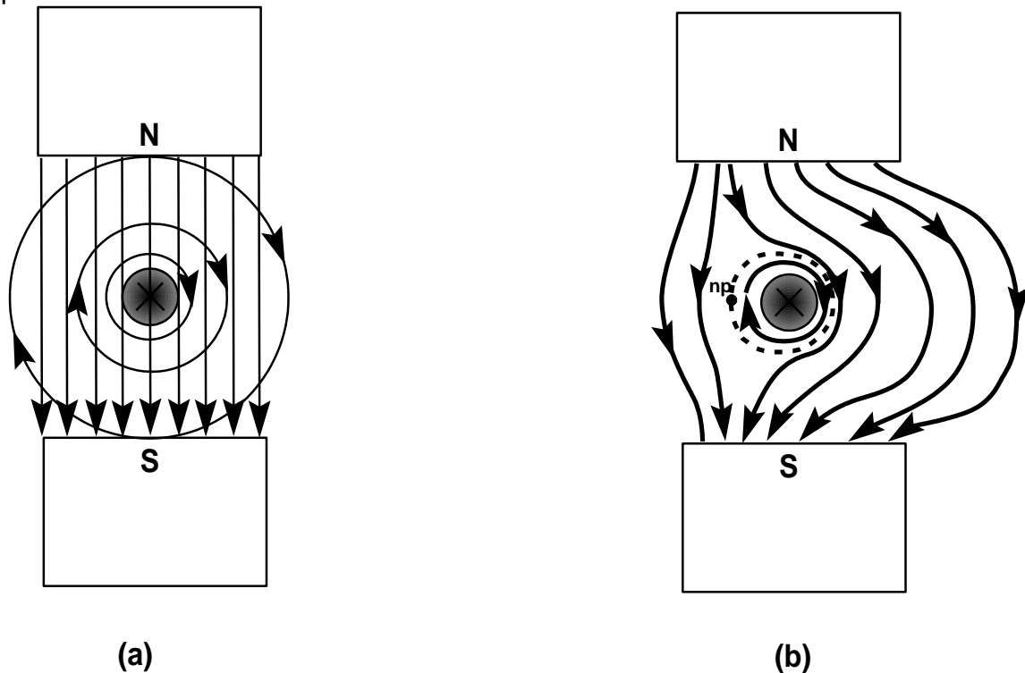
Figure 1. Idealized sketch of the magnetic fields due to an air gap and a current carrying conductor. (a) The individual component fields. (b) Sketch of the resulting total field.
